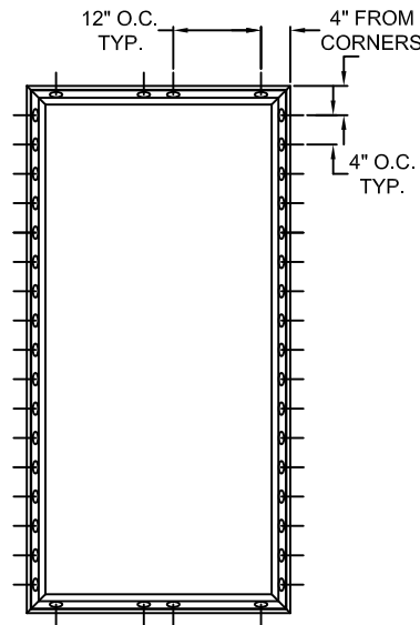
TYPICAL ELEVATION WITH FASTENER SPACING
